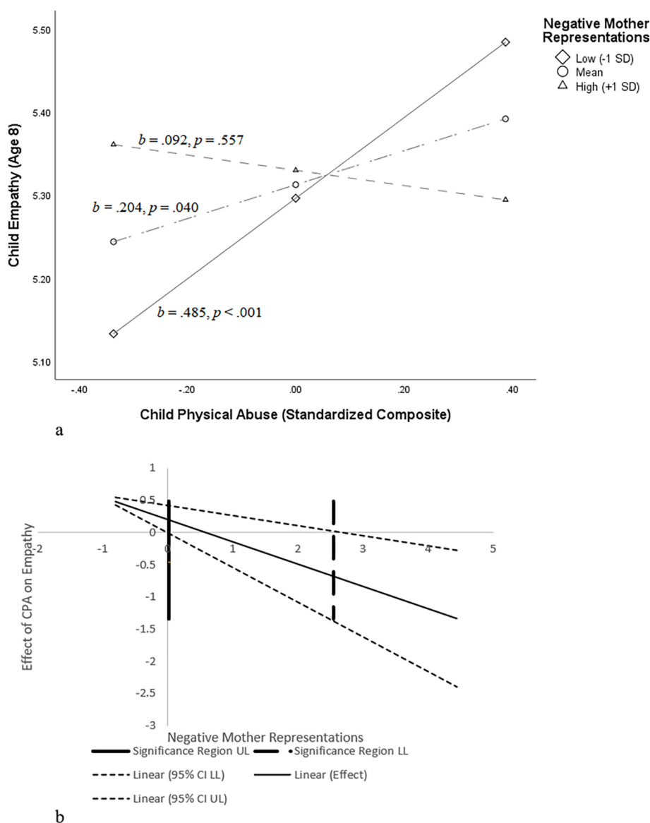
Fig. 1. a. Association between child physical abuse and child empathy as moderated by negative mother representations.
